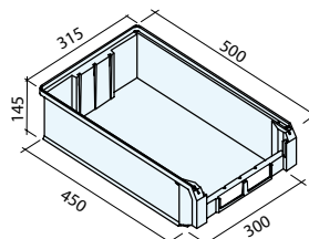
Art. PM5751 (OP-4A2) Dim. 500/450x300x145h mm Cap. 20 litros
