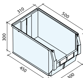
Art. PM7351 (OP-4A5) Dim. 500/450x300x300h mm Cap. 42 litros
