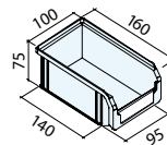
Art. PM1751 (OP-1) Dim. 160/140x95x75h mm Cap. 1 litros
