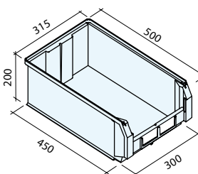
Art. PM6551 (OP-4) Dim. 500/450x300x200h mm Cap. 28 litros
