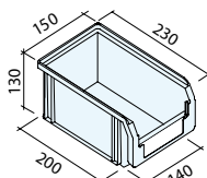
Art. PM2551 (OP-2) Dim. 230/200x140x130h mm Cap. 3,8 litros
