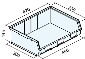
Art. PL4951 (OP-3L5) Dim. 350/300x450x145h mm Cap. 19 litros
