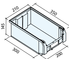
Art. PM3351 (OP-3A2) Dim. 350/300x200x145h mm Cap. 9,4 litros
