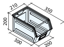
Art. LS4100 (OPM-3) Dim. 350/300x200x200h mm Cap. 12,5 litros
