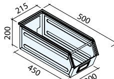
Art. LS4900 (OPM-3P4) Dim. 500/450x200x200h mm Cap. 18 litros
