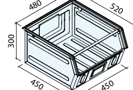
Art. LS8100 (OPM-5P4) Dim. 520/450x450x300h mm Cap. 63 litros
