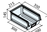
Art. LS3300 (OPM-3A2) Dim. 350/300x200x145h mm Cap. 9,4 litros
