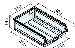
Art. LS5700 (OPM-4A2) Dim. 500/450x300x145h mm Cap. 20 litros
