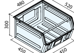
Art. LS8100 (OPM-5P4) Dim. 520/450x450x300h mm Cap. 63 litros
