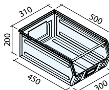
Art. LS6500 (OPM-4) Dim. 500/450x300x200h mm Cap. 28 litros
