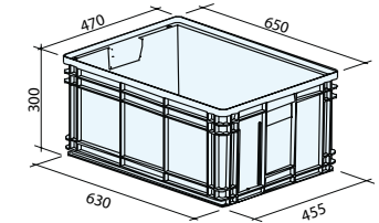
Art. PJ8951 (TR-5) 630x450x300h mm. Cap. 85 litros
