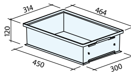
Art. PJ5751 (TR-4A2) 450x300x120h mm. Cap. 16,2 litros
