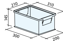
Art. PJ3351 (TR-3A2) 300x200x145h mm. Cap. 8,7 litros
