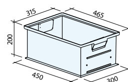
Art. PJ6551 (TR-4) 450x300x200h mm. Cap. 27 litros
