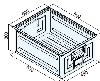
Art. LA8920 (TRM-5) Dim. 630x450x300h mm Cap. 85 litros
