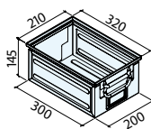
Art. LA3320 (TRM-3A2) Dim. 300x200x145h mm Cap. 8,7 litros
