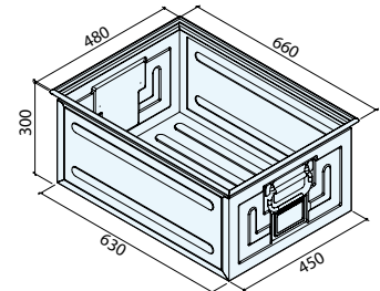
Art. LA8920 (TRM-5) Dim. 630x450x300h mm Cap. 85 litros
