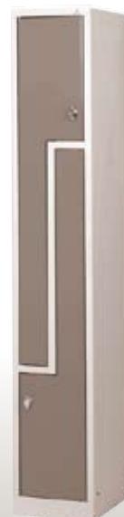
Art. PLM4-1x2 Dim. 400x500x1800h mm
