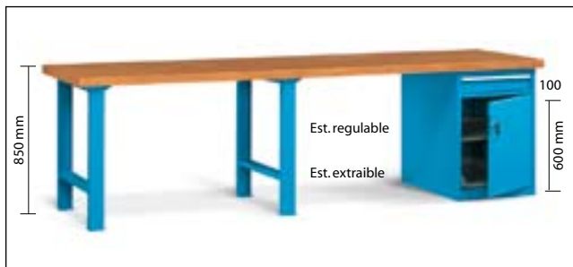
Art. M4-8030-19 (Dim. 3000x800x850h mm)
