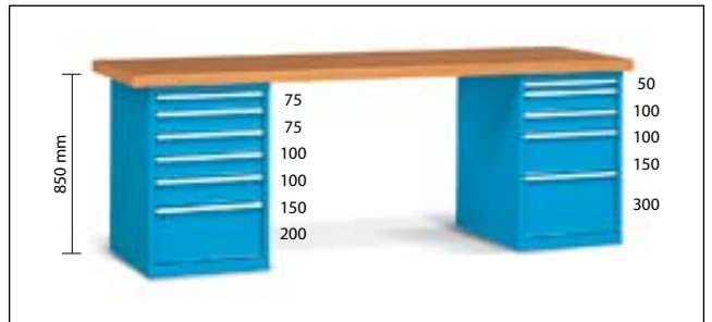
Art. M4-8025-17 (Dim. 2500x800x850h mm)
