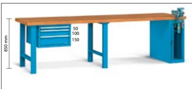
Art. M4-8030-37 (Dim. 3000x800x850h mm)
