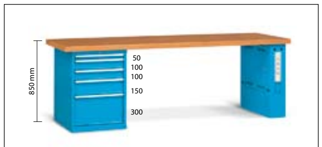
Art. M4-8025-50 (Dim. 2500x800x850h mm)
