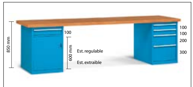
Art. M4-8030-31 (Dim. 3000x800x850h mm)
