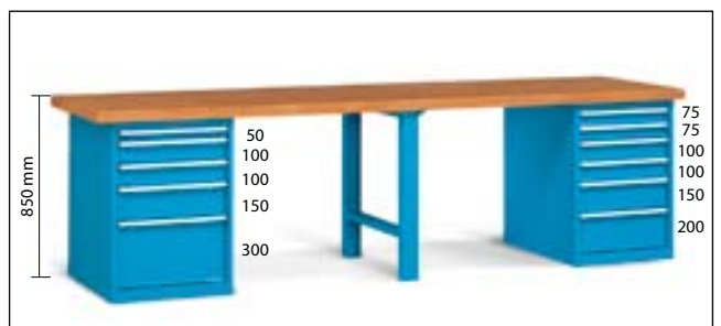
Art. M4-8030-17 (Dim. 3000x800x850h mm)
