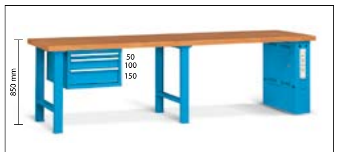
Art. M4-8030-46 (Dim. 3000x800x850h mm)
